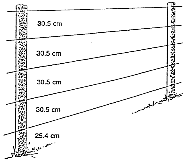
Fig. 8. Two-meter-high Penn State electrified deer fence (from Palmer et al. 1985).
