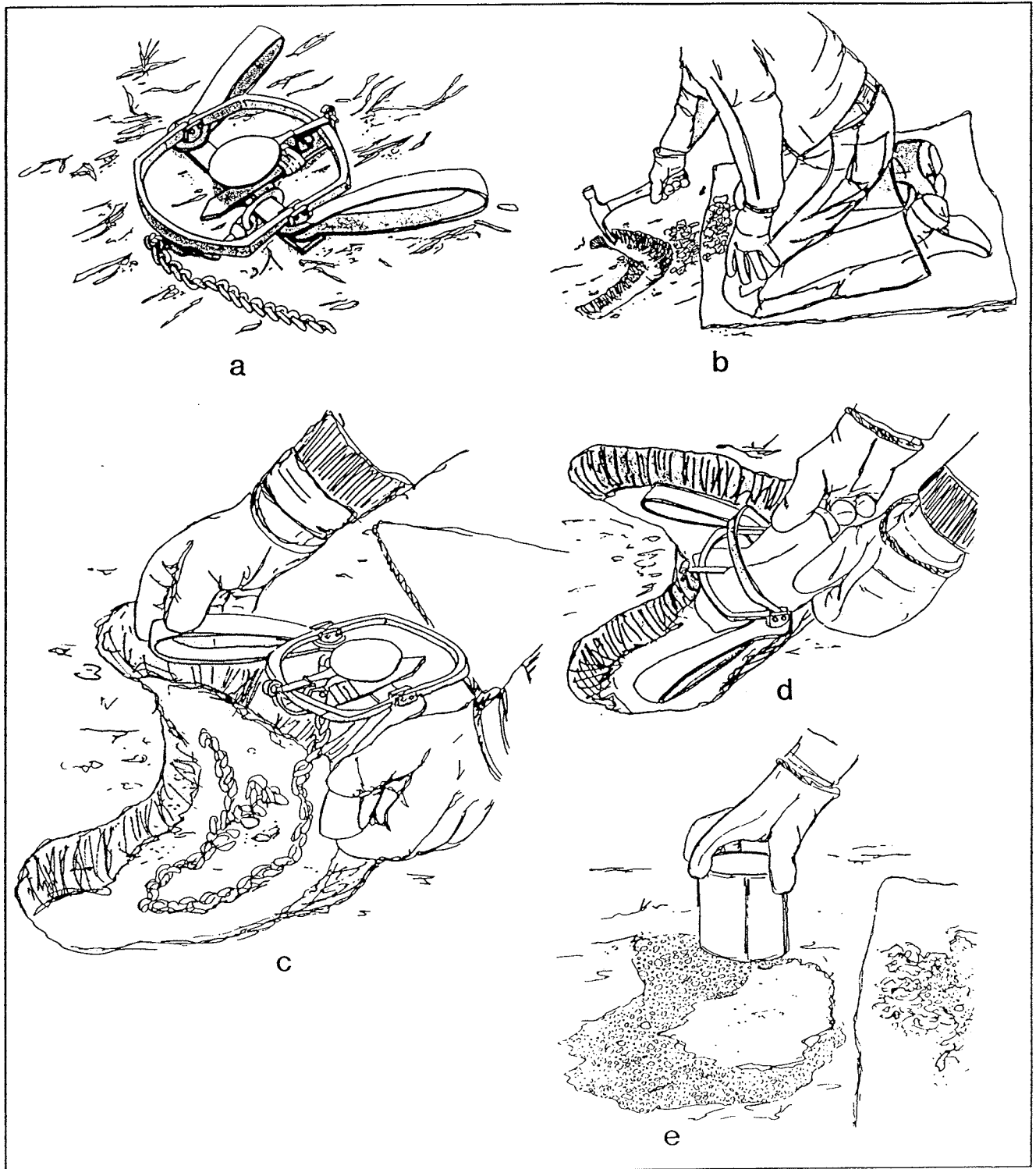
Fig. 18. a. A leg-hold trap is first laid on the ground to determine best location of hole. b. The hole should be about 11 cm deep and shaped to accommodate the trap. c. If a stake is used, it is driven into the bottom of the hole. If a drag is used, it is placed in the hole. The chain is then put into the hole and covered with soil until the hole is about 3 cm deep and packed to provide a firm foundation. d. The front jaw is raised and the pan cover is placed over the pan so soil cannot get under the pan. e. The trap is covered with finely sifted soil to a depth of 0.6–1.2 cm. A stick or whisk broom is used to touch up and make set appear as natural as possible (from Dorsett 1987).
