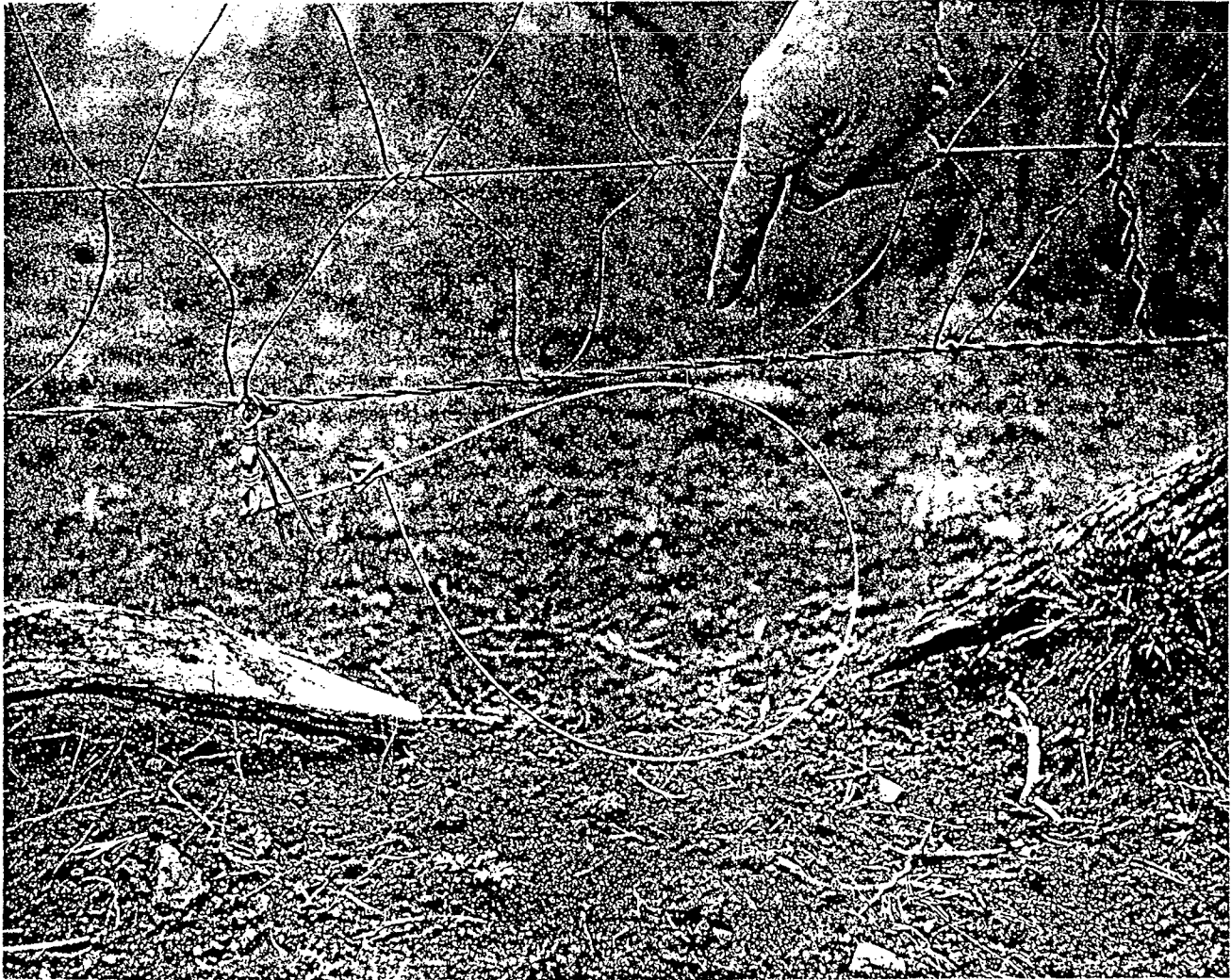
Fig. 17. The body snare, used primarily to capture coyotes, should be positioned directly under the fence with the top of the loop attached by a small, thin wire or a single strand of sewing thread. The attachment should release with the slightest pull (from Sims 1988).
