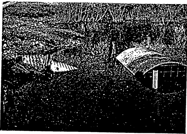
Fig. 12. Mechanical devices, such as these T-culverts developed in New York, may be used to prevent beavers from stopping water flow through culverts (photo, K. Roblee, N.Y. State Div. Fish Wildl.).
