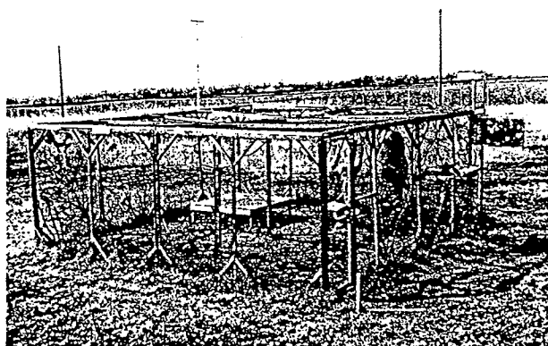
Fig. 6. A typical blackbird and starling decoy trap showing elevated feed platform in center and gathering cage on far right. Birds fold their wings to enter the trap through a 0.6- × 1.2-m opening covered with 5- × 10-cm welded wire located directly above the feed platform (photo, R. A. Dolbeer).
