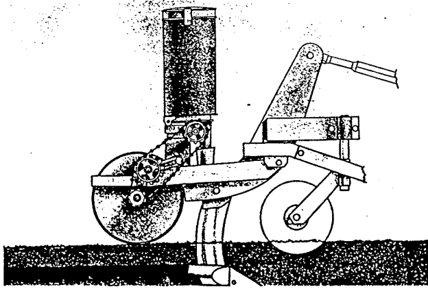
Fig. 13. Burrow builders are tractor-drawn mechanical devices used to create an artificial underground burrow and place toxic grain baits therein for controlling pocket gophers. Gophers intersect these burrows during their normal activity, feed on the bait, and die underground (sketch courtesy of Univ. California, Davis).
