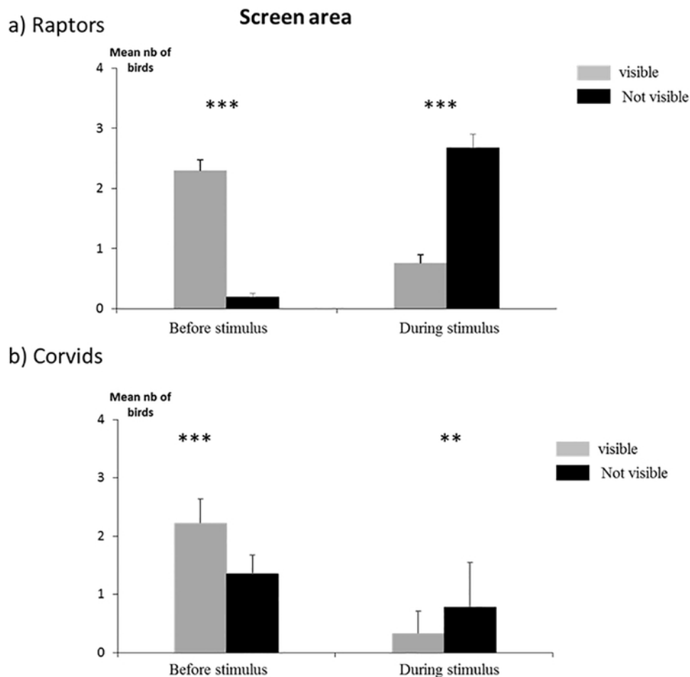
Fig 5. Numbers of birds in the screen area. (a: raptors, b: corvids) Numbers of birds in the screen area during the last week (before) pre-stimulus and the first week (during) the stimulus was presented for zones with or without access to the stimuli (mean per scan). Chi-square tests, *** p < 0.001 ( n = 121 scans for the 2 weeks).
