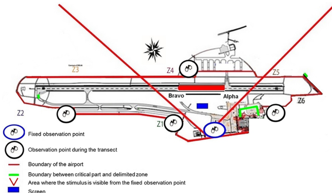
Fig 3. Map of the airport. a) transects used for the “entire airport” assessment. The stimuli could be seen at some places within Z1 and Z6 from a distance ( > 400 m), red squares: places where observers made recordings; b) the screen area seen from the fixed observation post (within the oblique red lines), the section of the runway where the risk of collisions is the greatest lies between alpha and bravo, blue rectangle: screens.
