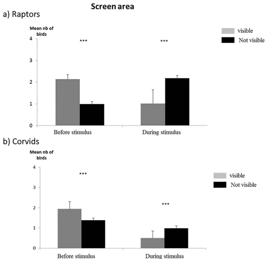
Fig 6. Distribution of birds. Distribution of birds over the whole study period: a) raptors and b) corvids over the screen area before and during display of the stimulus and according to visibility (mean number per scan). Chi-square test, *** p < 0.001 ( n = 288 scans for the whole period).
