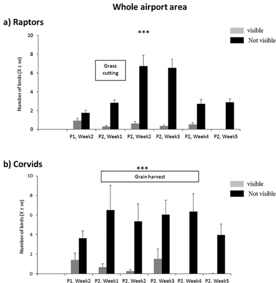
Fig 4. Number of birds along the transect. Numbers of birds (a: raptors, b: corvids) observed along the airport transects in relation to visual access to the stimulus (mean per scan). Chi-square test; *** p < 0.001 ( n = 239 scans for the whole study period).
