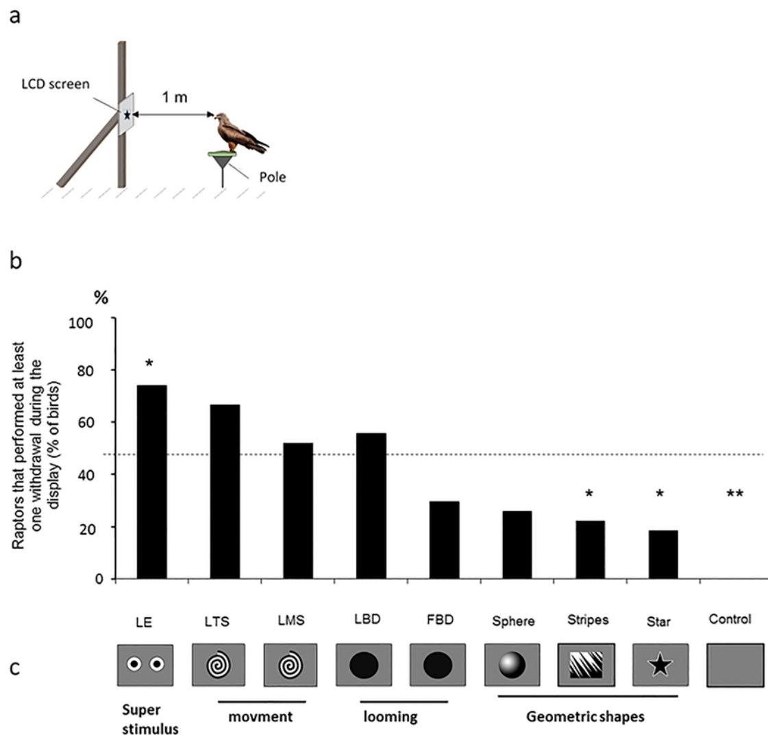
Fig 1. Captive study. a) test apparatus; b) birds (in percent) that reacted to the display of the visual stimulus. c) stimuli: LE: looming eyes, LTS: looming turning spiral (as used on some aircraft), LMS: looming moving spiral, LBD: looming black disc, FBD: static black disc, F Sph: static geometric shapes: sphere (depth impression), S: stripes (used for repelling birds from windows) [35], Fstar: static star, C control: grey screen. Chi-square test, * p < 0.05 ; c) The stimulus displayed: LE: looming eyes, looming turning (LTS) versus moving (LMS) spiral, looming (LBD) versus static (FBD) black disc, static geometric shapes: sphere (F Sph), strips (S) static star (Fstar) and control (C).
